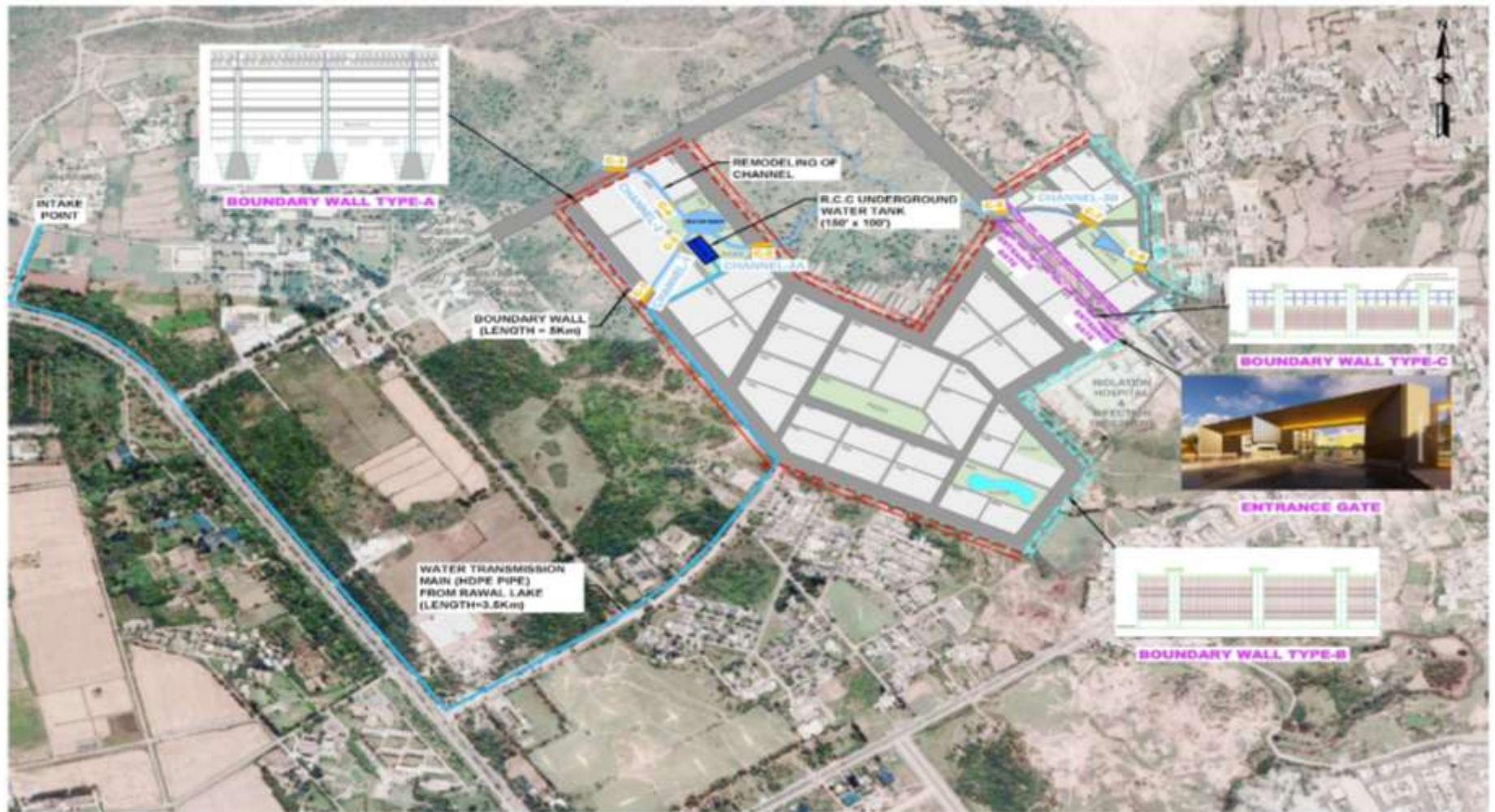
Figure 1.2: Layout Plan of Proposed Components
